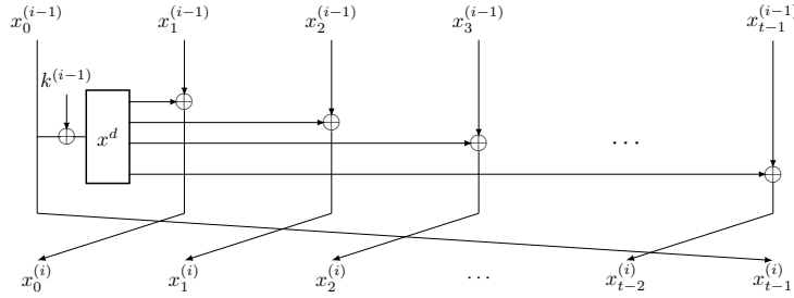
Fig. 4: The round function of \text{GMiMC}(n, t) .
