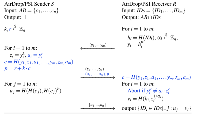
Figure 3: Maliciously secure PSI protocol of [54] applied to DO2 (cf. § 4.2). The non-interactive zero-knowledge AND-proof of knowledge is marked in blue [16, 37, 86].
