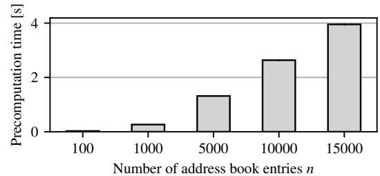
Figure 10: Runtime of PSI precomputation on an iPhone 12.
