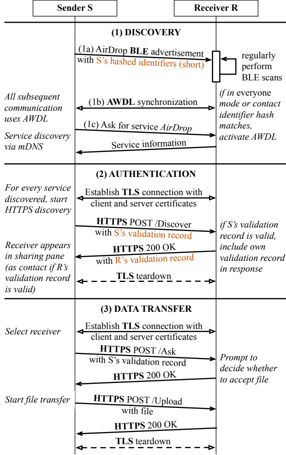
Figure 1: AirDrop protocol (simplified version from [93]). The orange message parts leak the sender’s and receiver’s contact identifiers, as discussed in § 3.3 and § 3.4, respectively.
