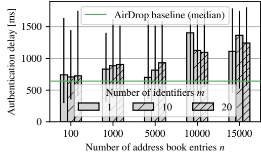
Figure 9: Overall authentication delay for AirDrop (baseline) and PrivateDrop with different set sizes (m, n) (MacBook Pro 2019 → iPhone 12 via AWDL).
