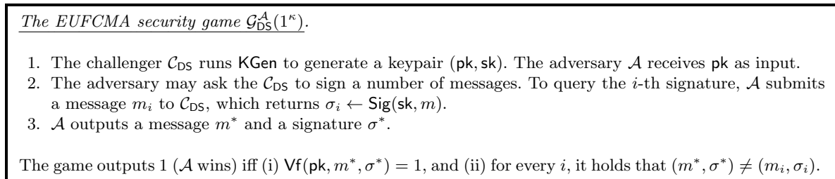
Fig. 1. The EUFCA security game \mathcal{G}_{\text{DS}}^{\text{A}}(1^\kappa) between the challenger \mathcal{C}_{\text{DS}} and the adversary \mathcal{A} .
