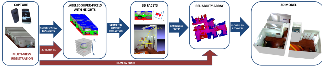
Figure 1: Method pipeline. Starting from few overlapping spherical images, we recover sparse 3D features and registered cameras. Such global information is used to enrich a per-image labeling into wall, ceiling and floor-superpixels, to robustly create 3D facets and segmentation reliability maps. A fusion approach finally generates a global 3D model.
