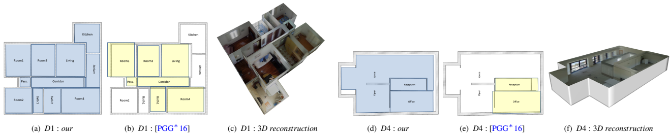
Figure 4: Recovered footprint and 3D models vs. ground truth floor plan. Comparisons against real, metrically scaled, ground truth (grey footprint), of our method (first column) and the multi-room approach of Pintore et al. [PGG*16] (second column). We show in the third column our final textured 3D floor plan. Ceilings and septal wall have been removed from 3D reconstruction to make the illustration more clear.
