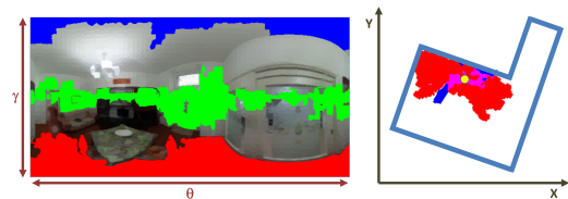
Figure 2: Image segmentation and resulting facets. Left: our super-pixels conservative segmentation. Right: the same ceiling and floor super-pixels represented as facets (see Sec. 3.2).
