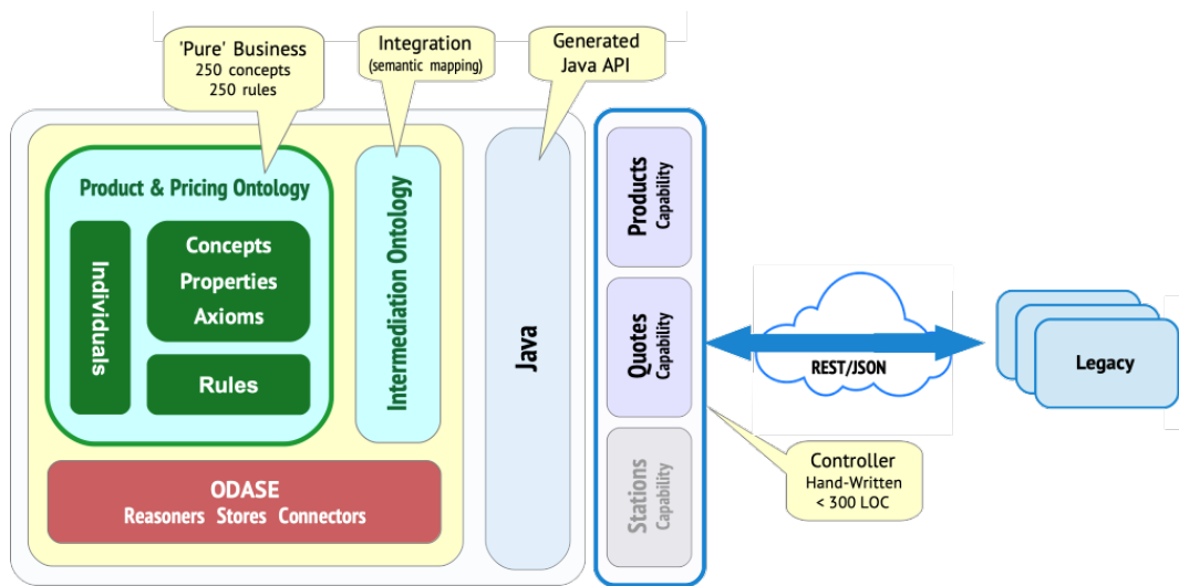
Figure 4: Software architecture
