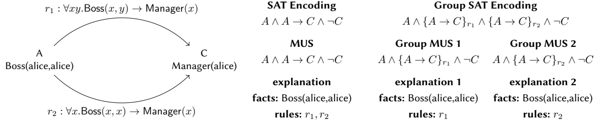
Figure 2: SAT vs Group-SAT Translation Example
