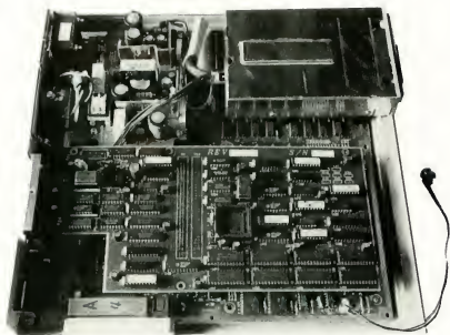
Figure 1. The Moniterm adapter board plugs easily into the Mega bus port. Once you manage to get inside the Mego, the rest is easy.
