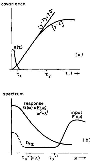
Fig. 2. Input and response of stochastically forced (single component) climate model with linear feedback; (a) covariances, (b) spectra. In the ranges \tau_x \ll \tau < \tau_y and \tau_y^{-1} \ll \omega \ll \tau_x^{-1} the models with and without feedback are identical. In the range \omega \leq \tau_y^{-1} the spectrum F(\omega) cannot be regarded as part of the "weather input", but is coupled to the climate response.
