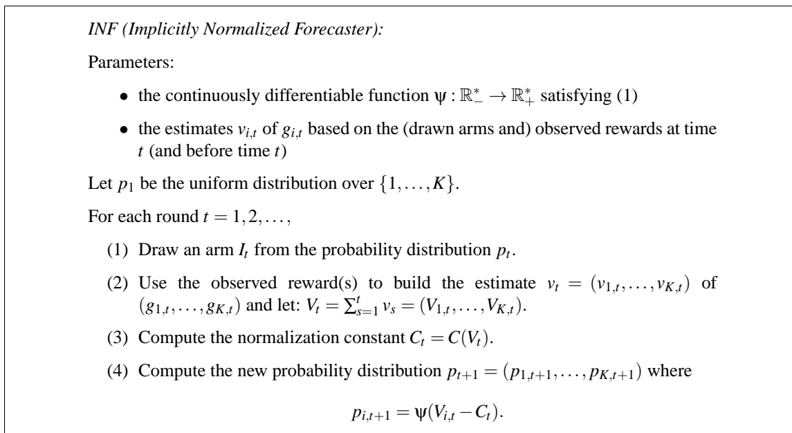
Figure 2: The proposed policy for the general prediction game.
